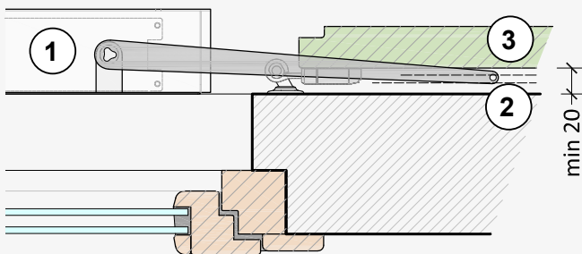
Type 1 Straight hinge banding to wall
