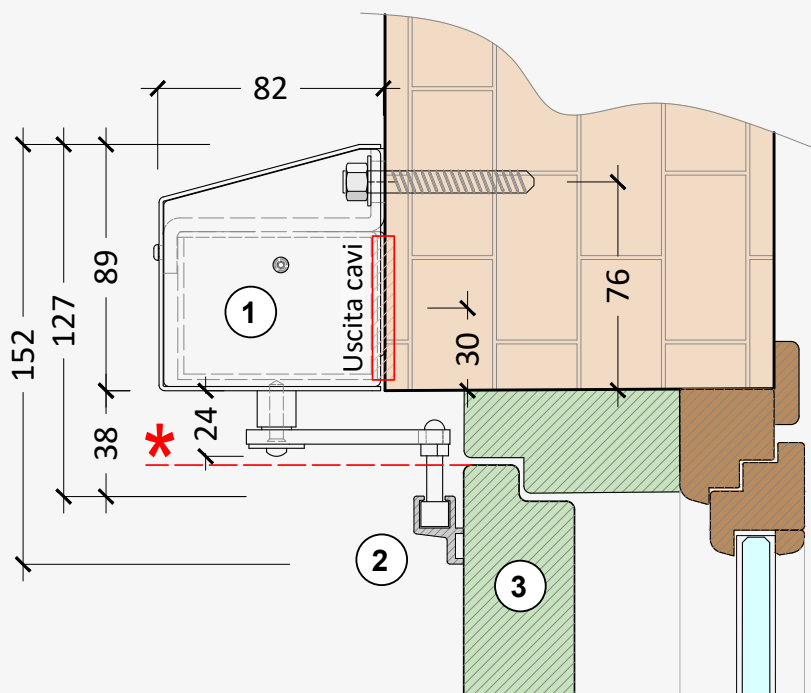
Door with rebate
