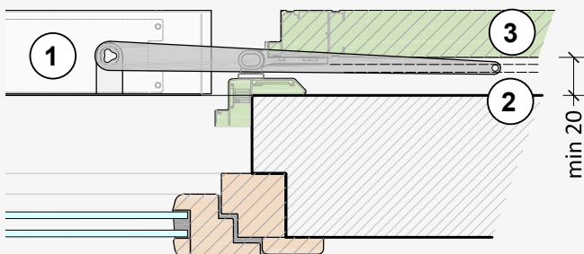
Type 2 Straight and hinge on aluminium frame
