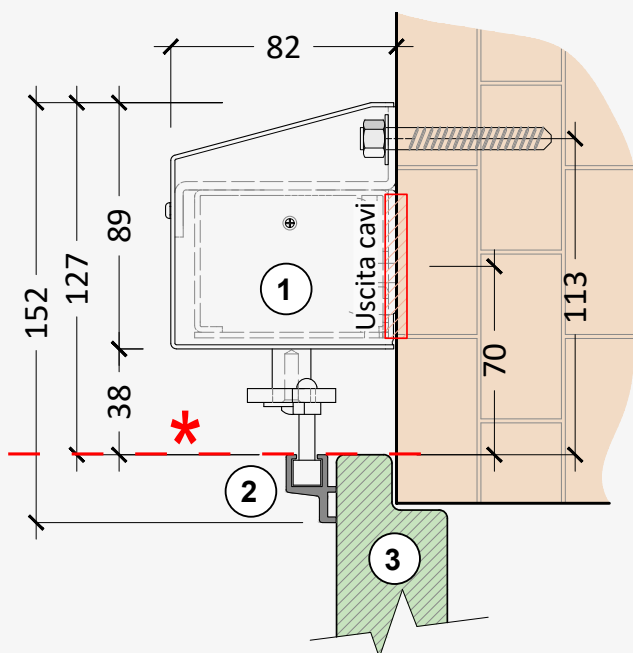
Traditional sash with rebate
