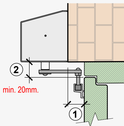
Wall-mounted overlay door no measures are necessary Colour specification required
