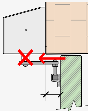
Flush-retracted door
