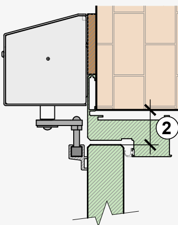
Sash on casing measure Pos.2 required Colour specification required
