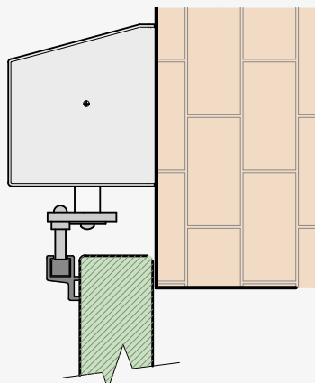
Wall-mounted door no measures are necessary Colour specification required
