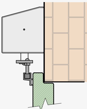
Wall-mounted overlay door no measures are necessary Colour specification required
