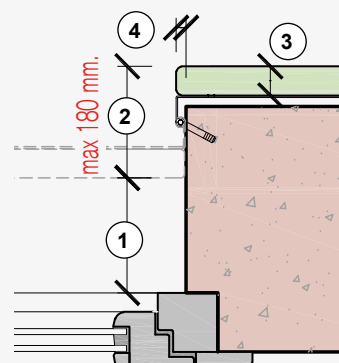
Hinge overhang on one-piece block with sash
