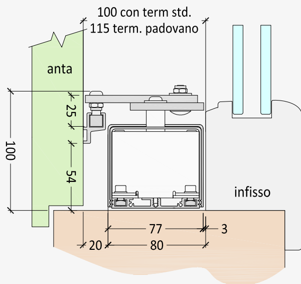
Side-by-side track
