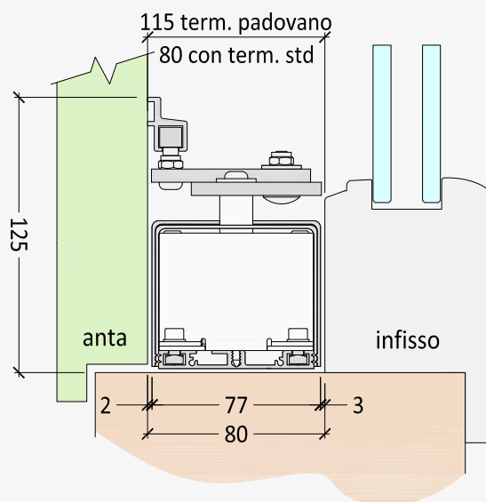
Overhead track
