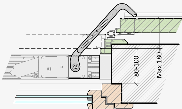
Type 2 Straight and hinge on aluminium frame
