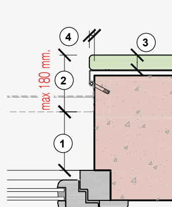
Hinge overhang on one-piece block with sash
