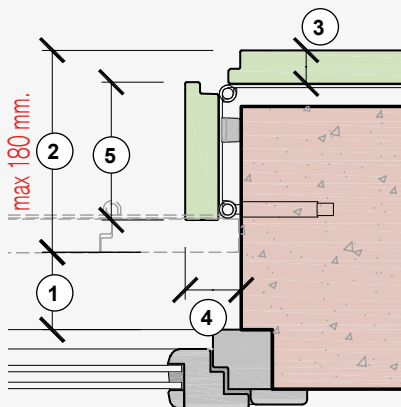
Straight hinge hinge rebated wooden sash
