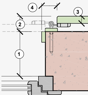
Straight hinge hinge rebated wooden sash
