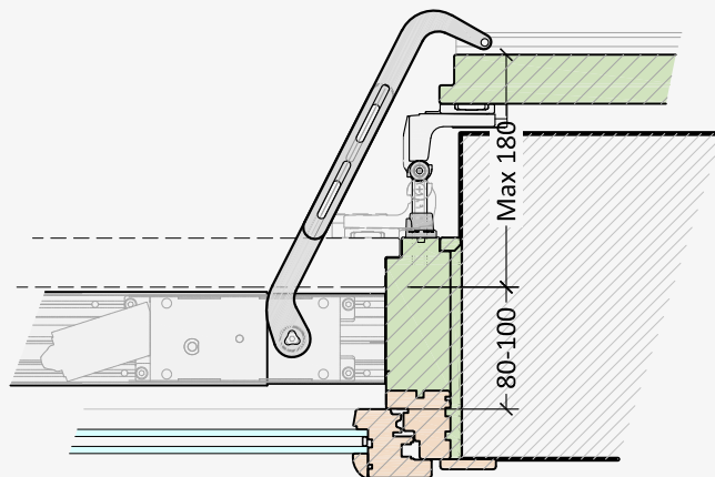
Type 4 Overhang on single block
