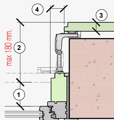
Hinge overhang on one-piece block with sash
