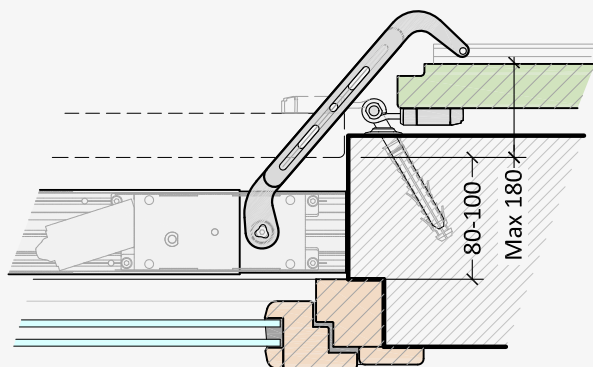
Type 1 Straight hinge strip
