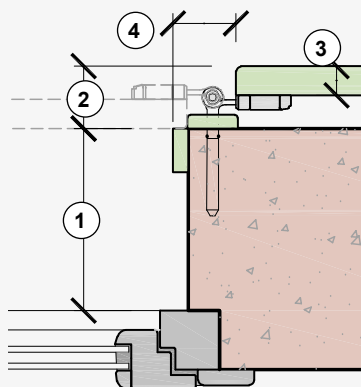
Straight hinge hinge wood door rabbet
