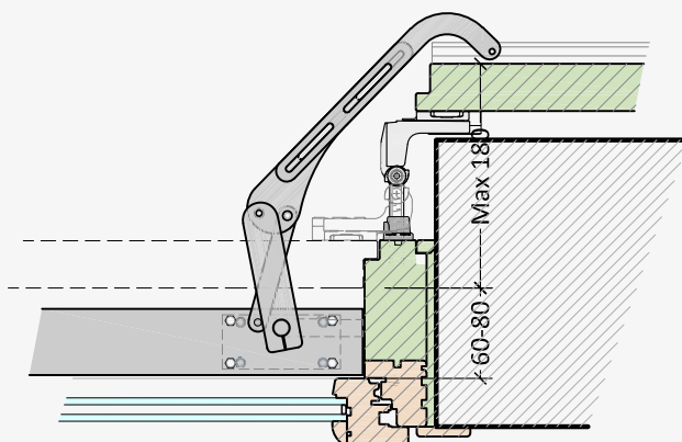
Type 4 Overhang on single block
