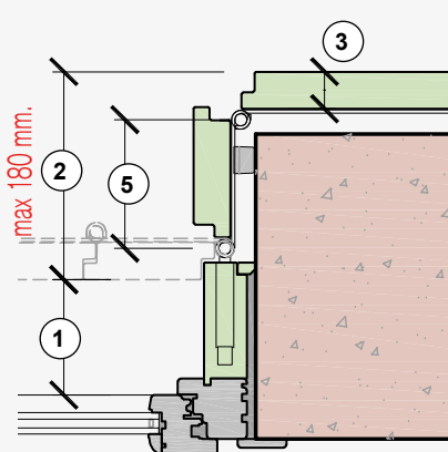
Straight hinge strip
