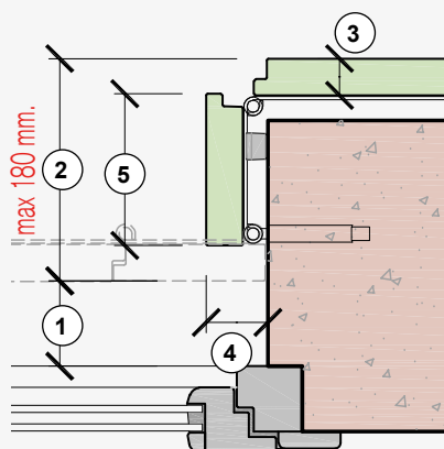
Straight hinge hinge wood door rabbet
