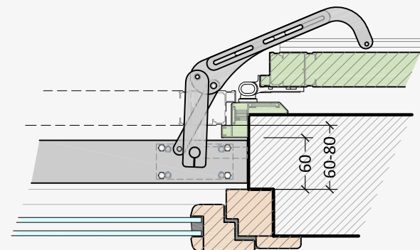
Type 2 Straight and hinge on aluminium frame
