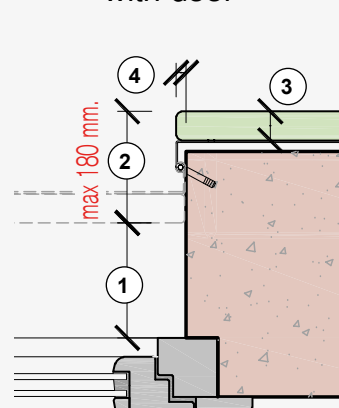
Hinge overhang on one-piece block with door
