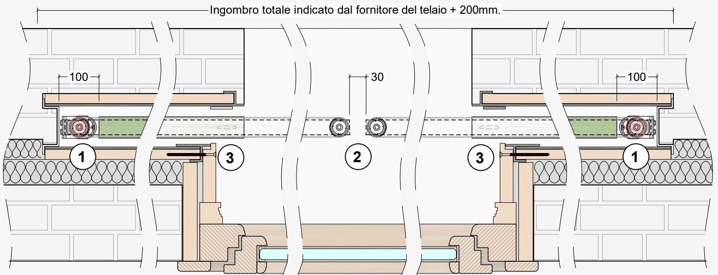
Application on double-door sliding counter frame
