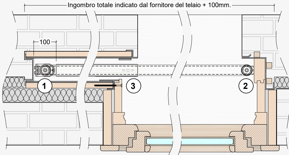
Application on single-door sliding counterframe
